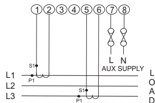
3 Phase 3 wire Unbalanced load
