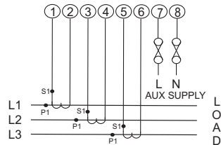
3 Phase 4 wire Unbalanced load
