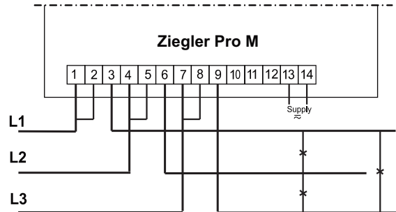
Direct measurement in a three-wire network.
