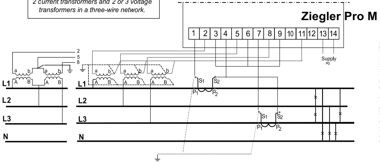
Fig 3. Electrical connections
